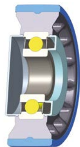
roller with cover and cover ring (CCR)
